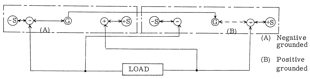
Fig. 3-8 Parallel connection diagram
