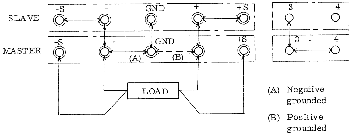
Fig. 3-11 Using sampling terminal in one-control parallel operation
